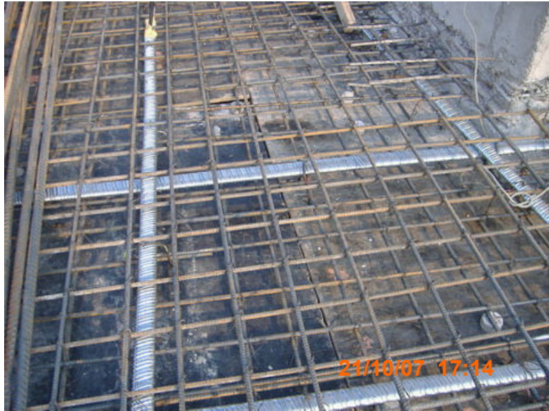
RE-BAR & POST-TENSION LEVEL 6 th
